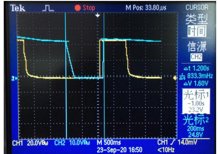
Output response & load (24V / 0.5A)
